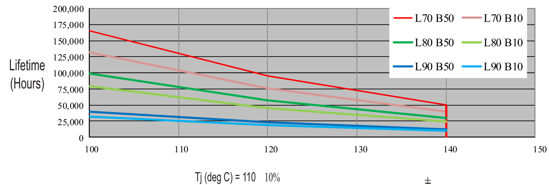
Lifetime for Citizen LED series - IF max 120mA/die
