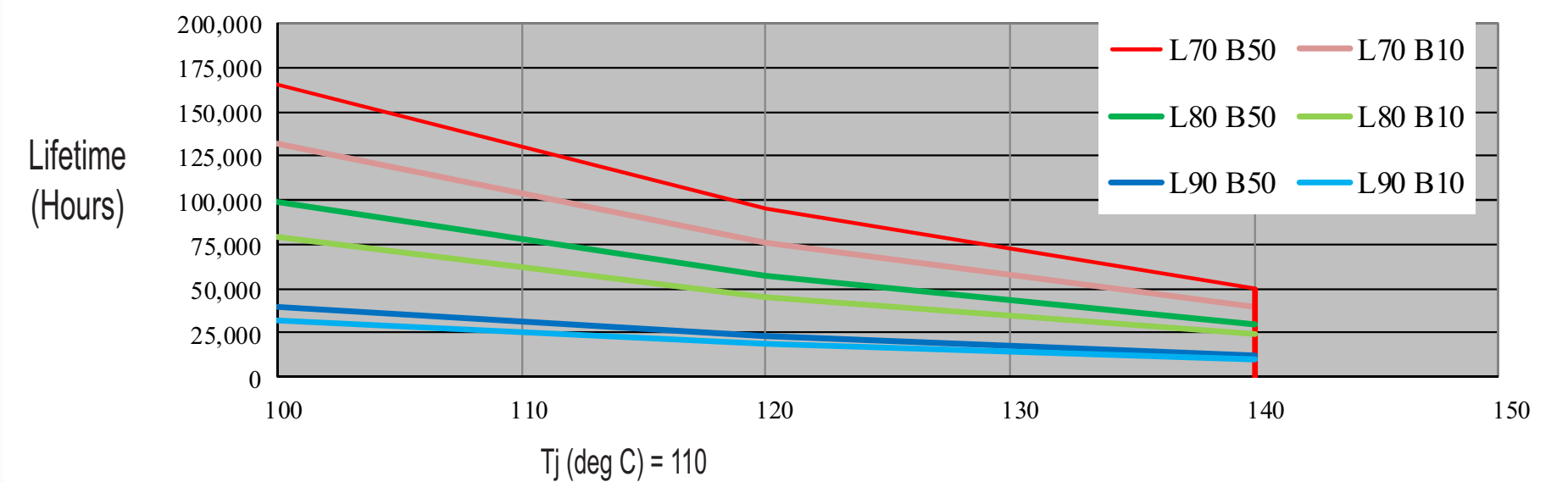
Lifetime for Citizen LED series - IF max 120mA/die
