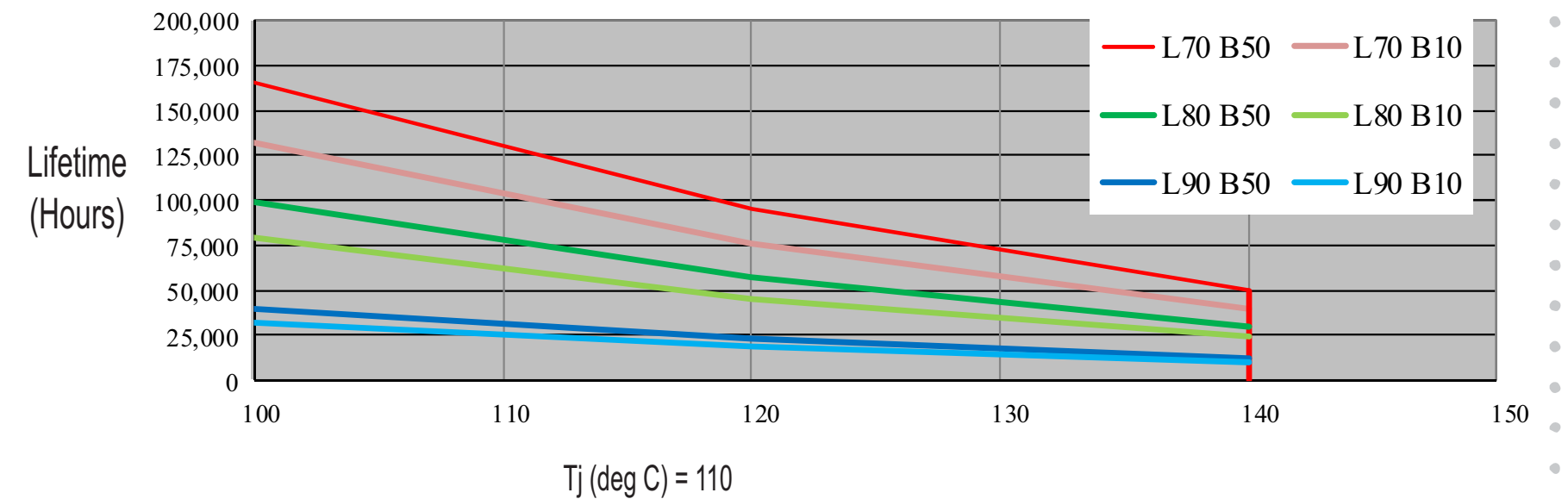
Lifetime for Citizen LED series - IF max 120mA/die
